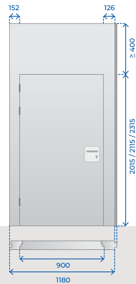
IPD Deur in paneel Inset Pass Door
