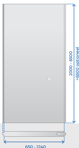
TP Telescoop paneel Telescopic Panel
